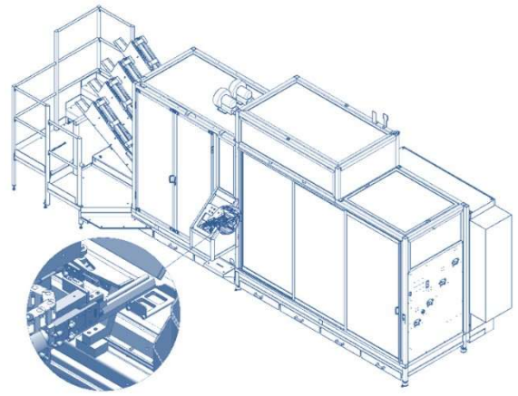
Parts mounted in the bag-folding area.
